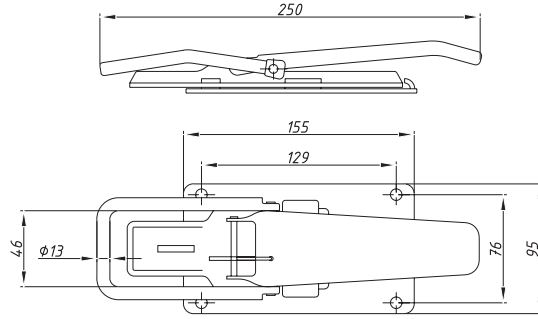
242200 Dorse Kiliti Düz Trailer Lock / Standard
