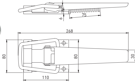
242100 Döküm Dorse Kiliti Trailer Lock / Casting
