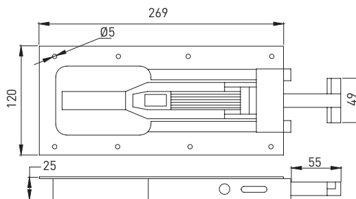
242400 Yeni Dorse Kiliti Gömme Trailer Mortise Lock / New
