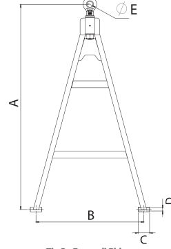
Tip 2 - Dereceli Okbaşı Type 2 - Towing Eye With Tube
